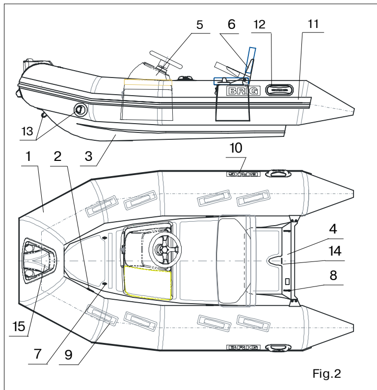
DELUXE version Boat General View (see Fig.2).
