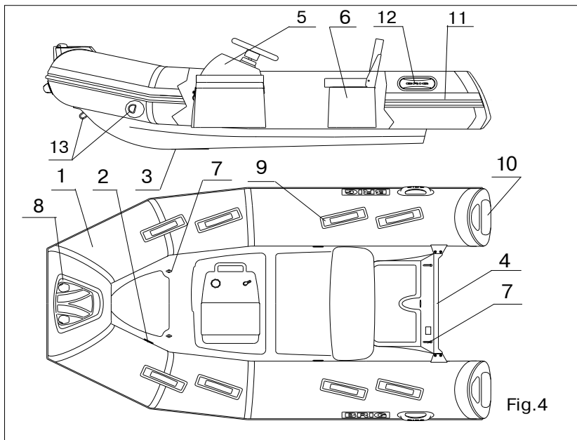
TENDER DELUXE version Boat General View (see Fig.4).
