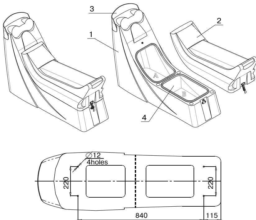
Fig.9 Sport console
