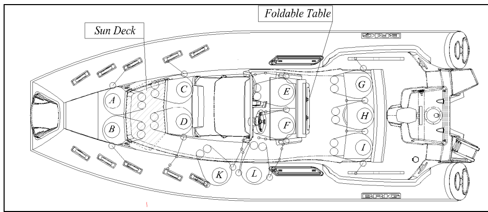
Fig.3a. Crew limit for Design Category C
