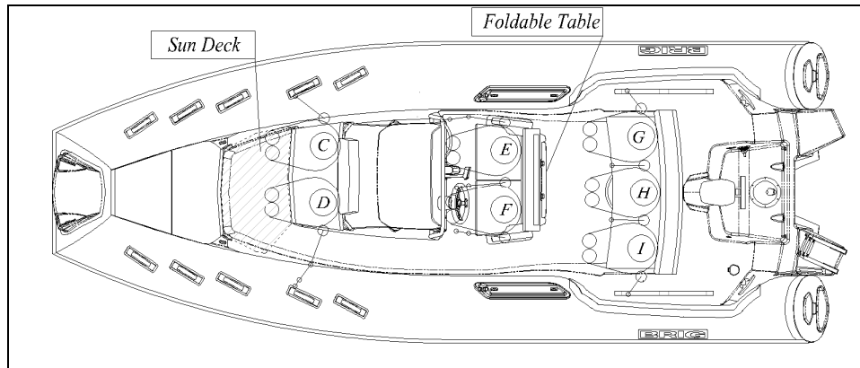
Fig.3b.Crew limit for Design Category B
